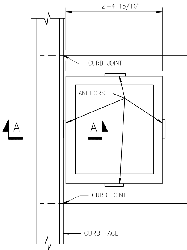
PLAN FOR PIPE 18" OR LESS
